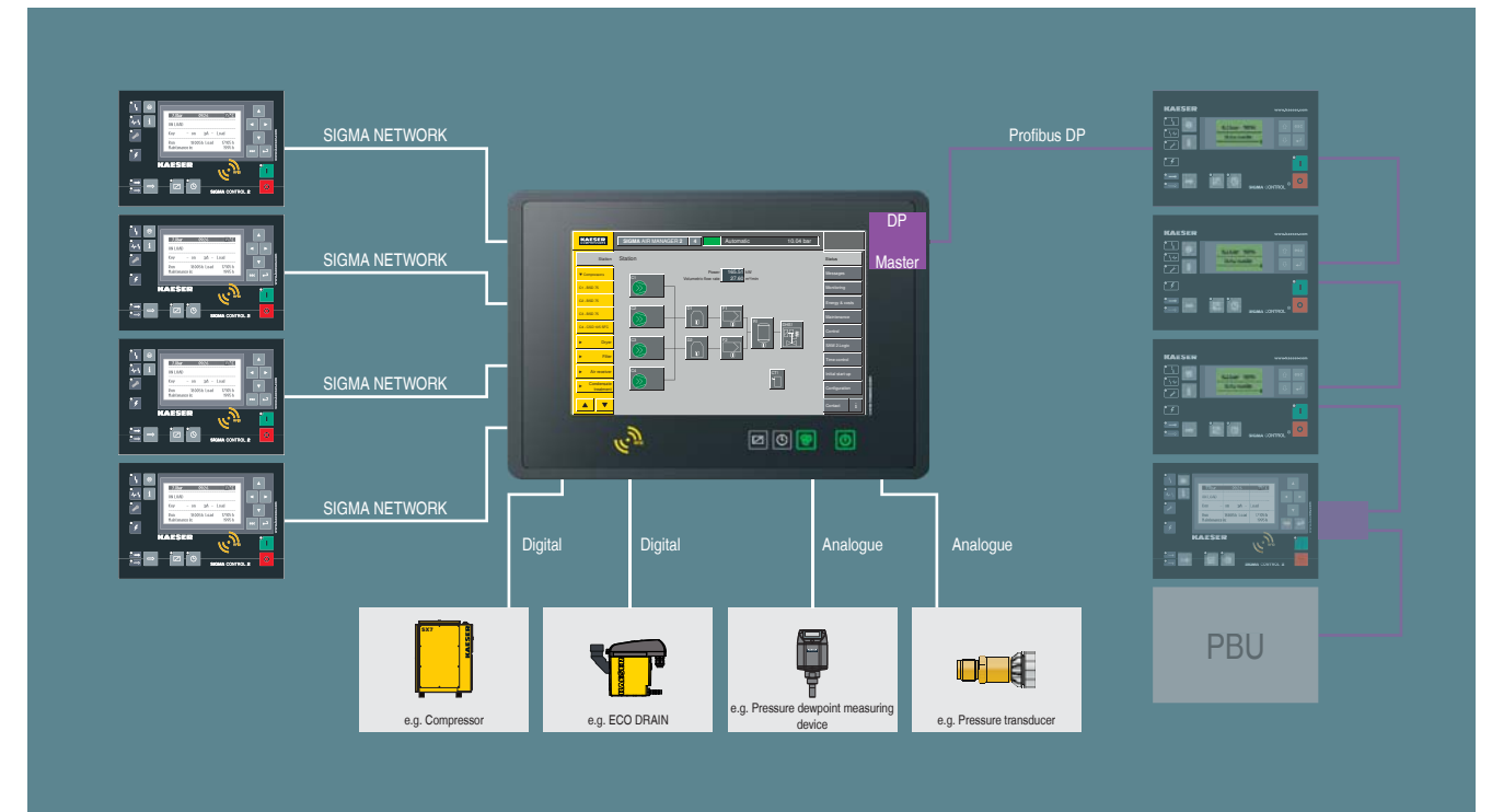
Compressed air station with SIGMA AIR MANAGER 2 – Possible connections
